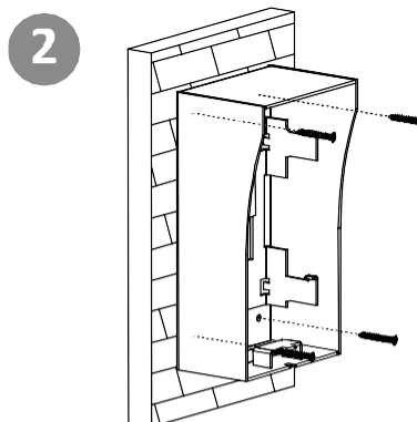
Affix the protective shield onto the wall with four screws.
