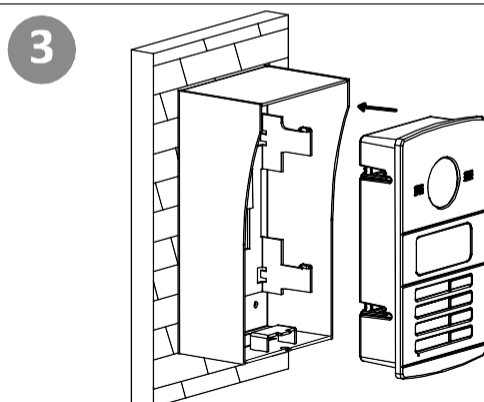
Install the door station onto part 1 of the protective shield.
