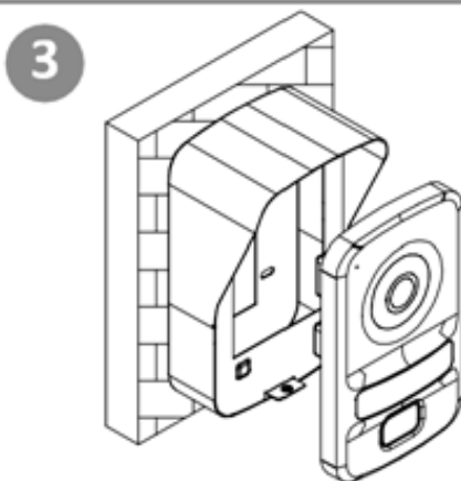
3 Install the door station into the protective shield.
